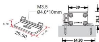
Mounting bracket
